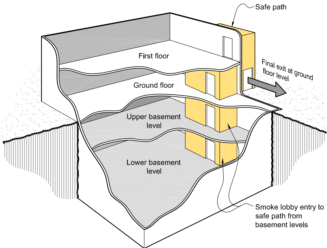
Figure 3.11 Single escape route from basement levels Paragraphs 3.5.2 and 3.13.1 f)
