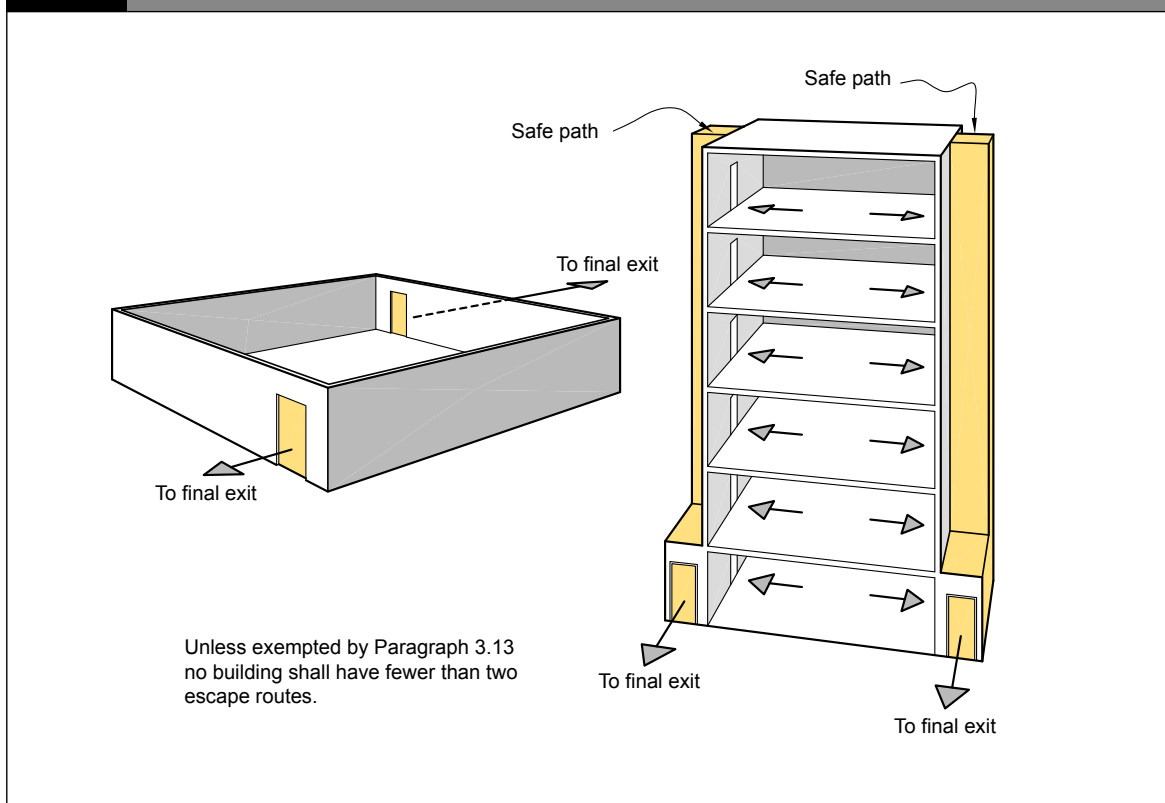
Figure 3.2 Minimum number of escape routes Paragraph 3.2.1
